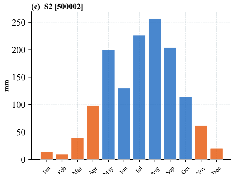
Figure 7. Monthly Rainfall Climatology — 1981–2014 Mean 1981–2014 | Wet Season: May–Oct | Dry Season: Nov–Apr
